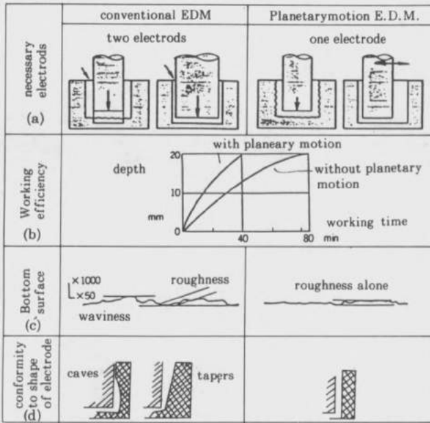
Fig. 6. - Advantages of planetary EDM (SAITO 1984).
