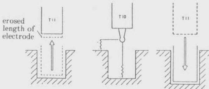
Fig. 7. - Principle of automatic tool wear compensation (SAITO 1984).
