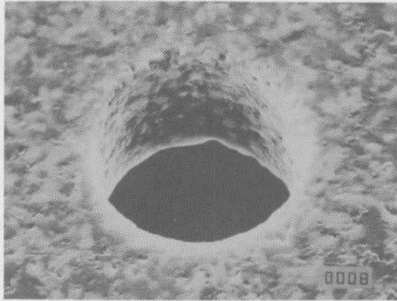
Fig. 4. — Micro Hole in TiB_2 - B_4C machined by EDM. Diameter 33 \mu m , thickness 45 \mu m (MASUZAWA 1986).
